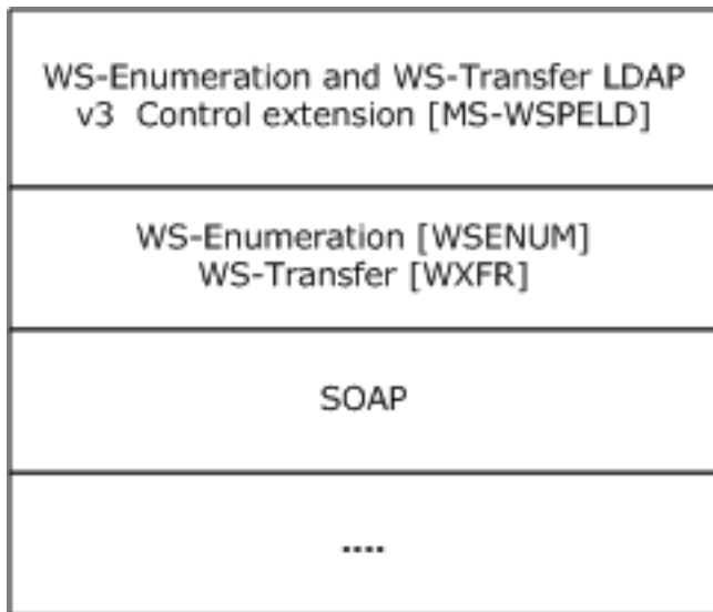
Figure 1: WPELD protocol stack
