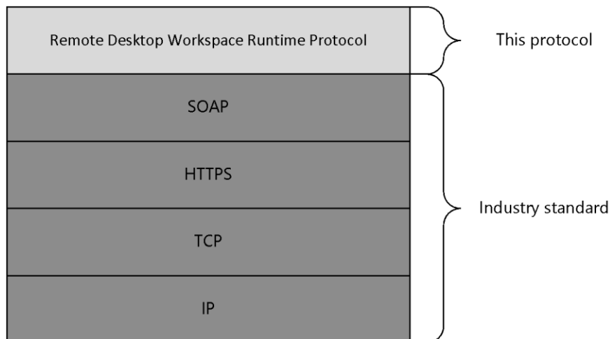
Figure 1: Protocol Stack
