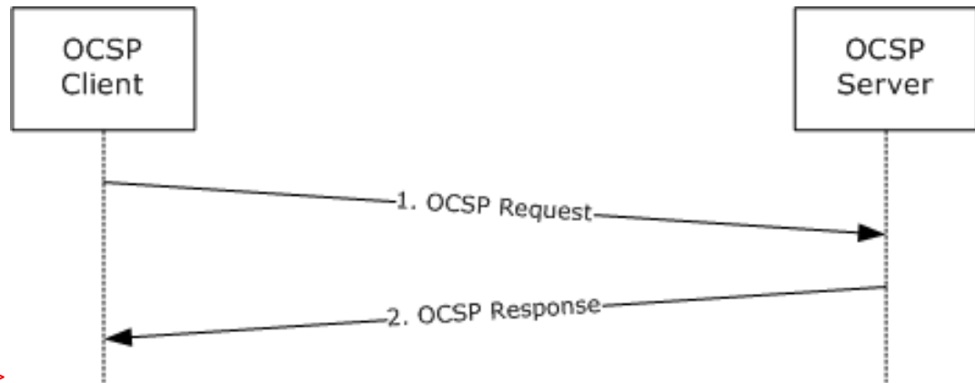
Figure 2: Revocation-checking process
