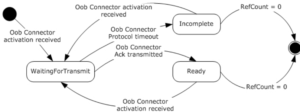
Figure 5: OoB Connector state transitions: Listener role
