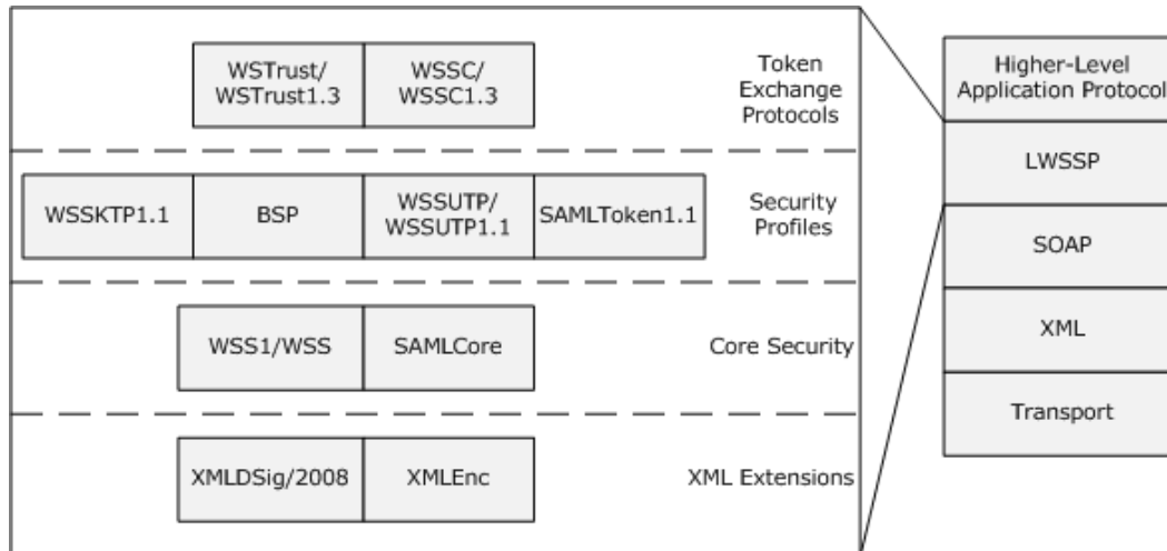
Figure 1: Protocol relationships
