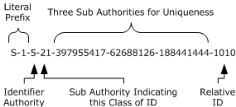
Figure 3: SID with account association
