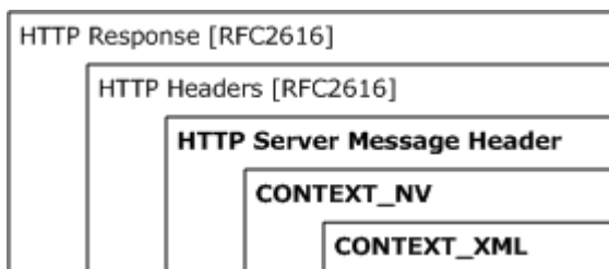
Figure 6: Server Context Establishing Message using HTTP 1.1
